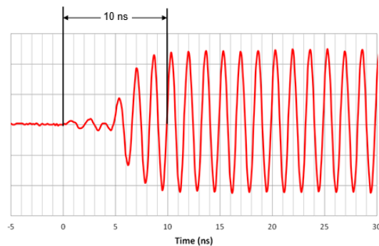
Figure 5: External Pulse Modulation Rise time
